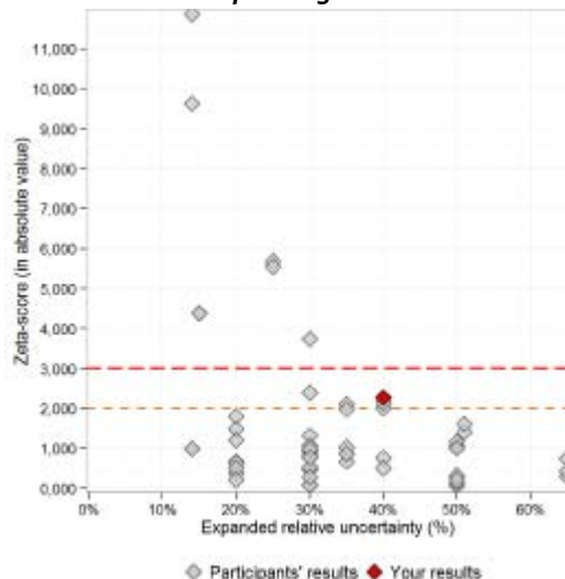
Zeta-score distribution depending on the uncertainties
